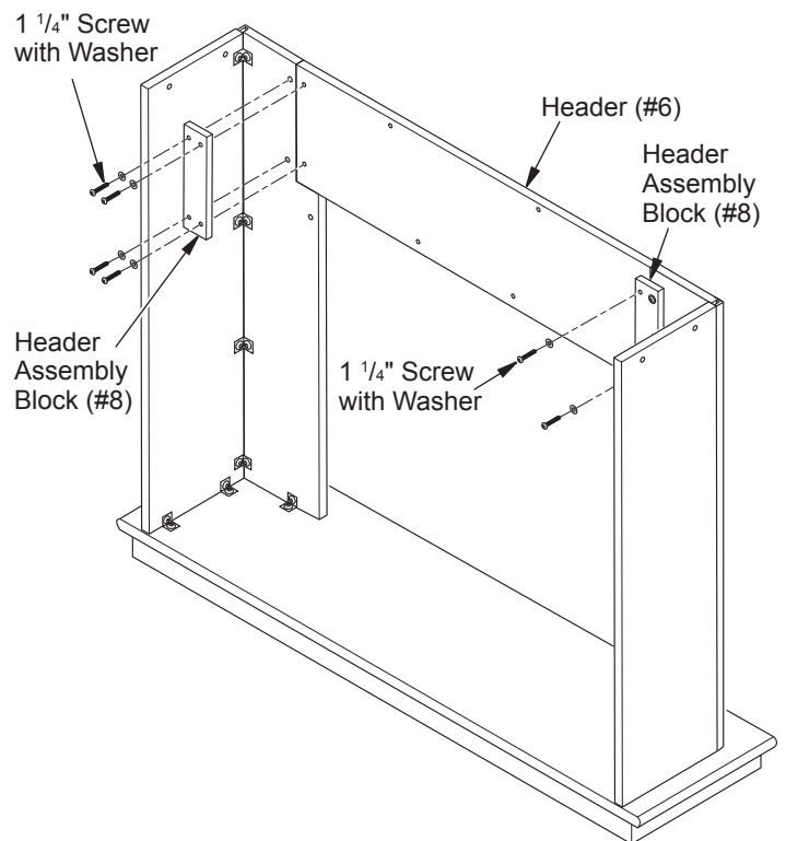
Figure 3 - Attaching Header
